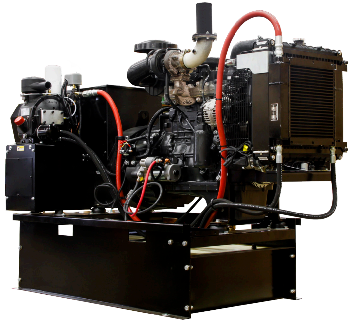
DE4040 - 40kW with 40 CFM @120 psi
